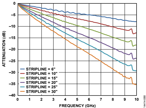
Figure 96. Insertion Loss of 50 Ω Striplines on FR4
