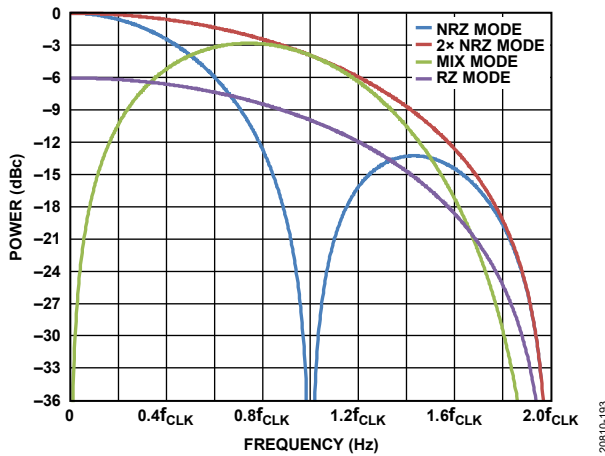
Figure 88. Sinc Roll-Off for 2x NRZ, NRZ, RZ, and Mix Mode Operation
