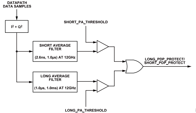
Figure 70. PDP Block Diagram
