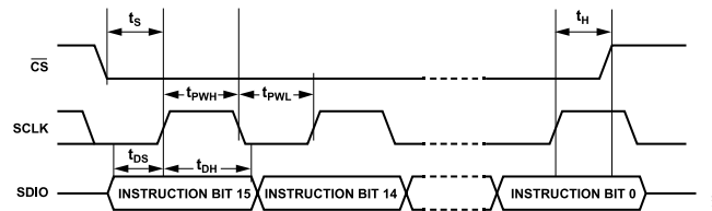
Figure 43. Timing Diagram for Serial Port Register Write
