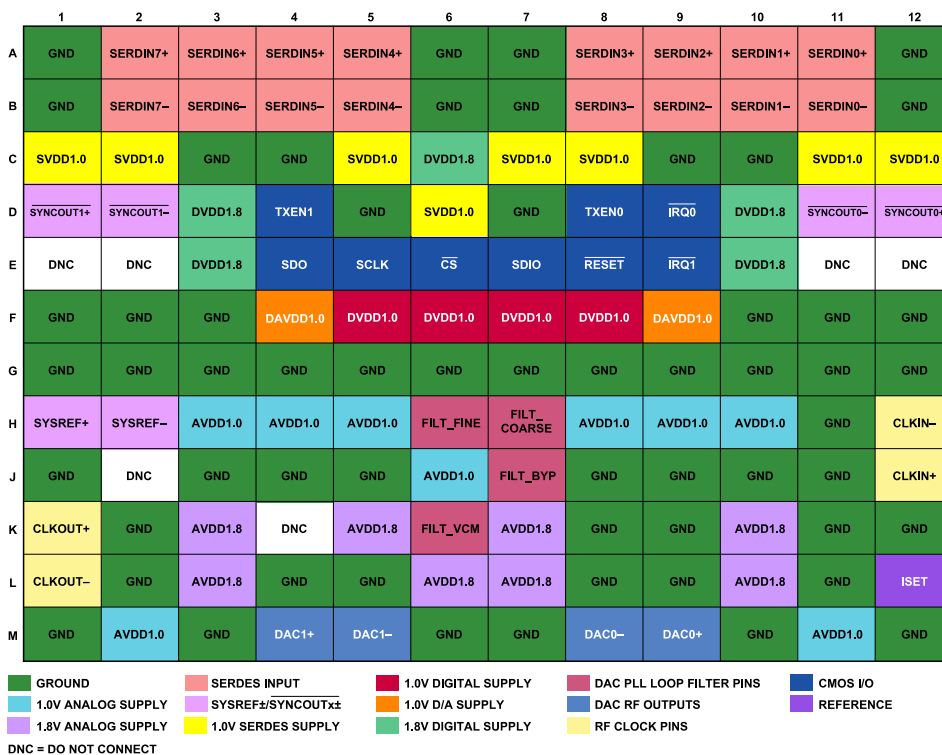
Figure 2. Pin Configuration
