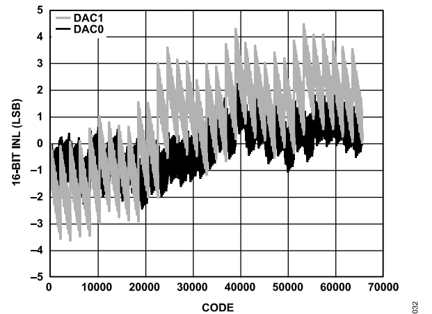
Figure 32. INL, I_{OUTFS} = 26 mA, 16-Bit Resolution
