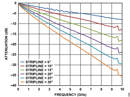
Figure 49. Insertion Loss of 50 Ohm Striplines on FR4
