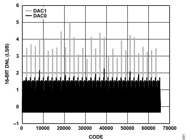
Figure 31. DNL, I_{OUTFS} = 26 mA, 16-Bit Resolution
