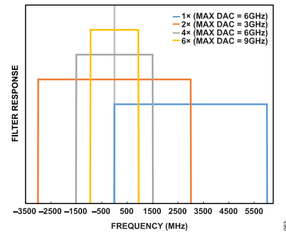
Figure 62. Band Responses of Total Interpolation Rates for 1x, 2x, 4x, and 6x at Each Respective Maximum Achievable DAC Rate
