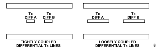
Figure 80. Tightly Coupled vs. Loosely Coupled Differential Traces
