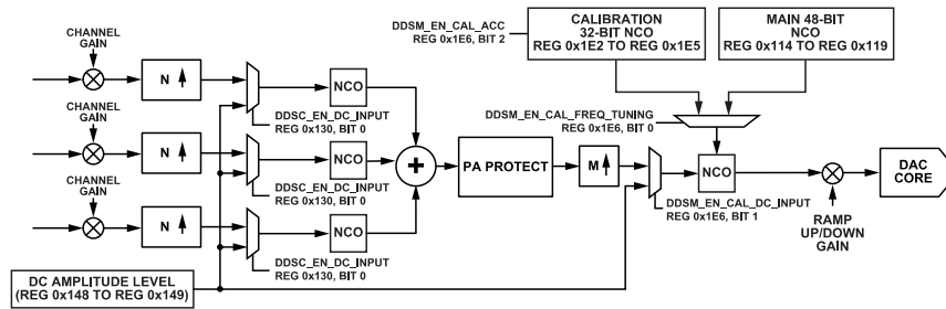
Figure 64. DC Amplitude Injection for NCO Only Mode Block Diagram
