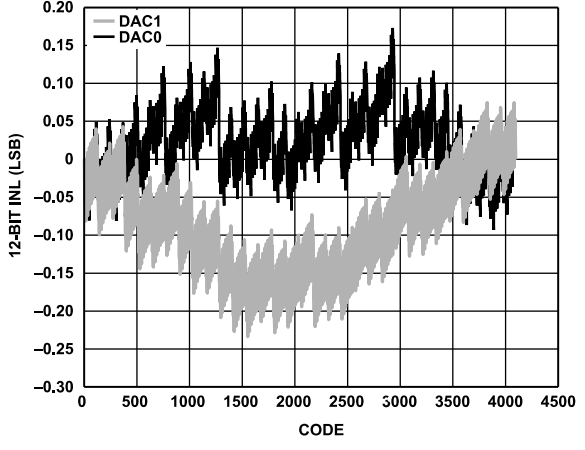
Figure 38. INL, I_{OUTFS} = 20\text{ mA} , 12-Bit Resolution
