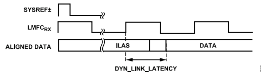
Figure 59. DYN_LINK_LATENCY_x Illustration
