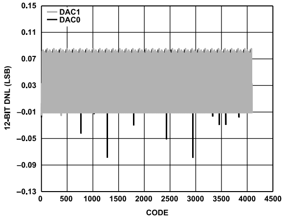
Figure 37. DNL, I_{OUTFS} = 20\text{ mA} , 12-Bit Resolution
