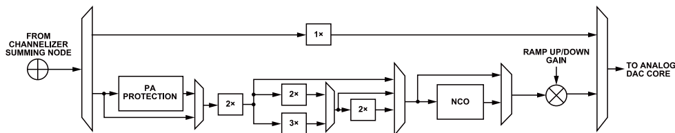
Figure 68. Block Diagram of the Main Digital Datapath per Main DAC Output
