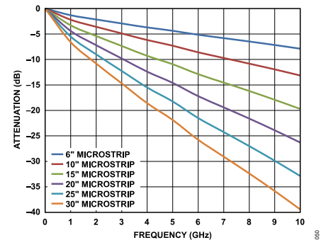
Figure 50. Insertion Loss of 50 Ohm Microstrips on FR4
