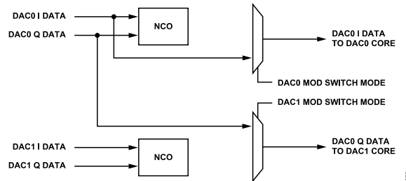
Figure 75. Mode 2—DAC0 = I0, DAC1 = Q0
