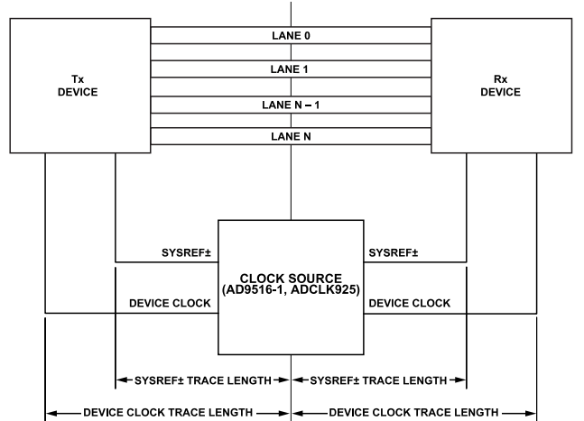
Figure 81. SYSREF± Signal and Device Clock Trace Length
