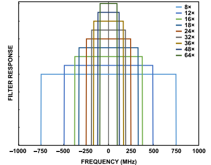
Figure 63. Band Responses of Total Interpolation Rates for 8x, 12x, 16x, 18x, 24x, 32x, 36x, 48x, and 64x at a 12 GHz DAC Rate
