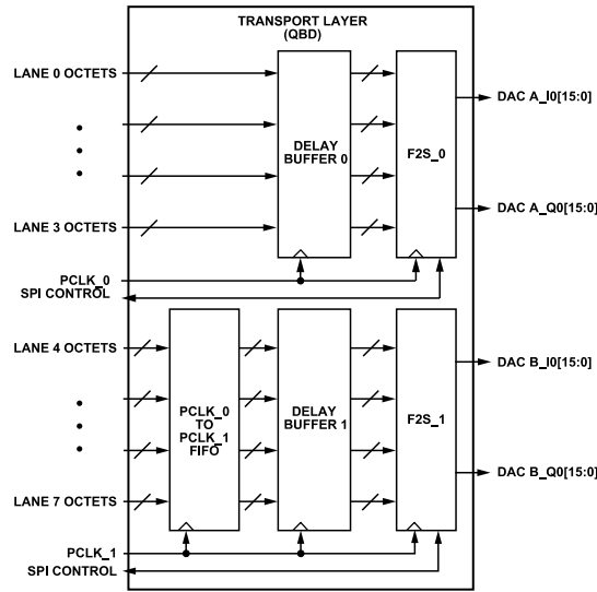
Figure 61. Transport Layer Block Diagram
