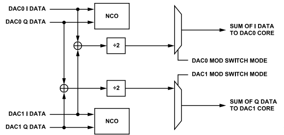
Figure 74. Mode 1—DAC0 = I0 + I1, DAC1 = Q0 + Q1
