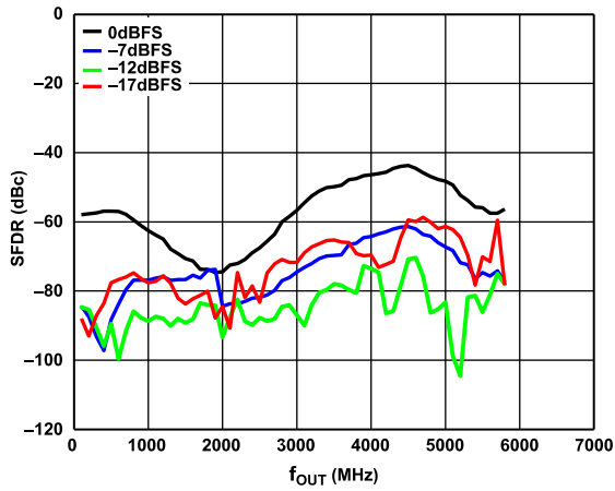
Figure 16. Third Harmonic (SFDR) vs. f_{OUT} over Digital Scale (Mode 9), 12 GHz DAC Sample Rate, Channel Interpolation 1x, Main Interpolation 8x
