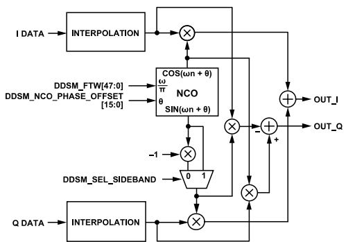
Figure 72. NCO Modulator Block Diagram
