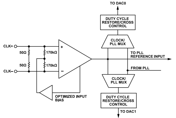
Figure 82. Clock Receiver Input Simplified Equivalent Circuit
