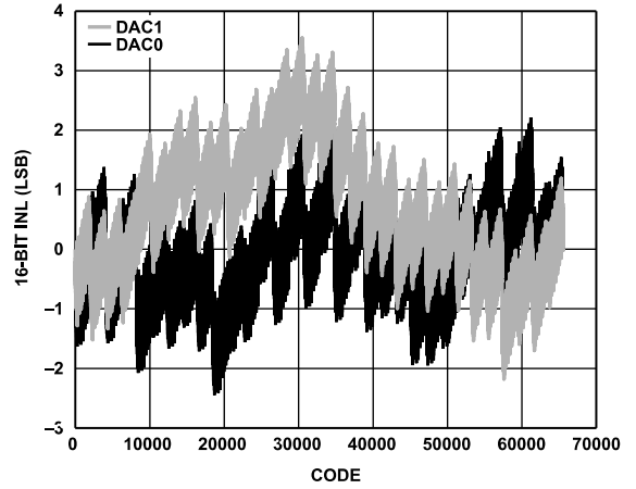
Figure 36. INL, I_{OUTFS} = 15.6\text{ mA} , 16-Bit Resolution
