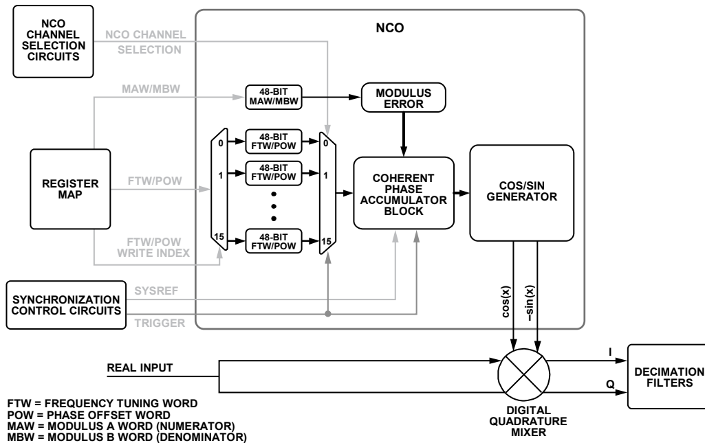
Figure 95. NCO and Mixer Block Diagram
