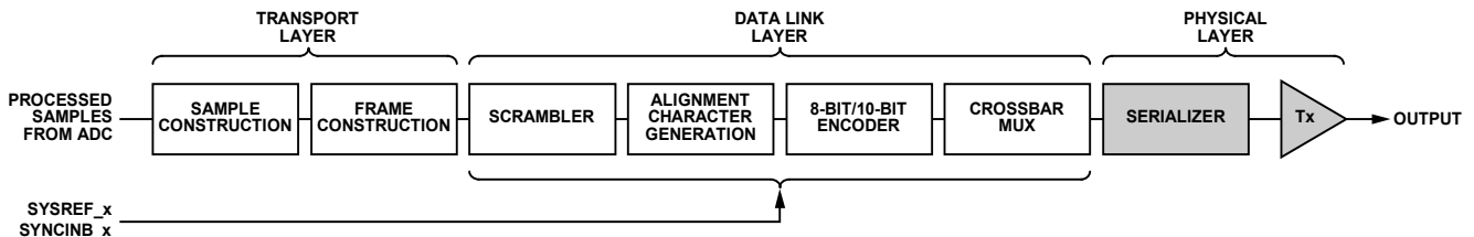
Figure 116. Data Flow
