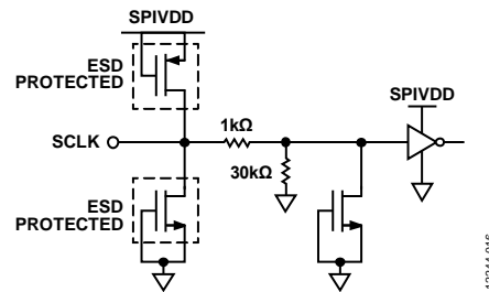
Figure 57. SCLK Input
