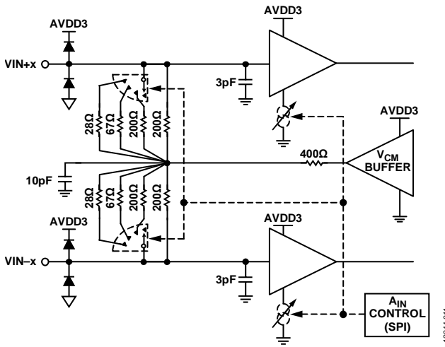
Figure 52. Analog Inputs
