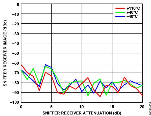
Figure 117. Sniffer Receiver Image vs. Sniffer Receiver Attenuation, 2600 MHz LO, CW Signal 1 MHz Offset, 20 MHz RF Bandwidth, 30.72 MSPS Sample Rate
