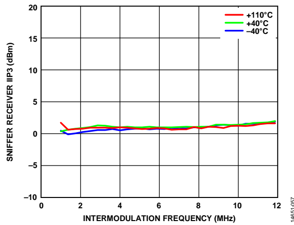
Figure 116. Sniffer Receiver IIP3 vs. Intermodulation Frequency ( f_2 - 2f_1 ), 2600 MHz LO, 0 dB Attenuation, 20 MHz RF Bandwidth, 30.72 MSPS Sample Rate
