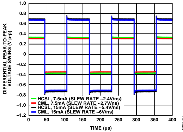
Figure 16. 8 kHz Output Waveforms for Various Driver Settings; HCSL Drivers Terminated 50 Ω to GND per Figure 32; CML Drivers Terminated 50 Ω to 1.8 V per Figure 33
