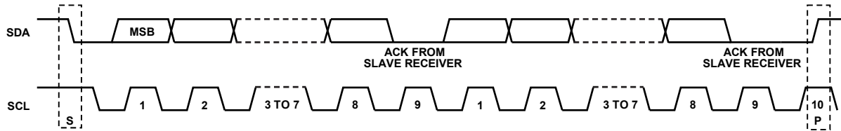
Figure 35. Acknowledge Bit
