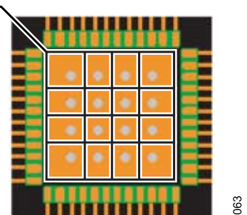
Figure 69. Typical PCB Layout
