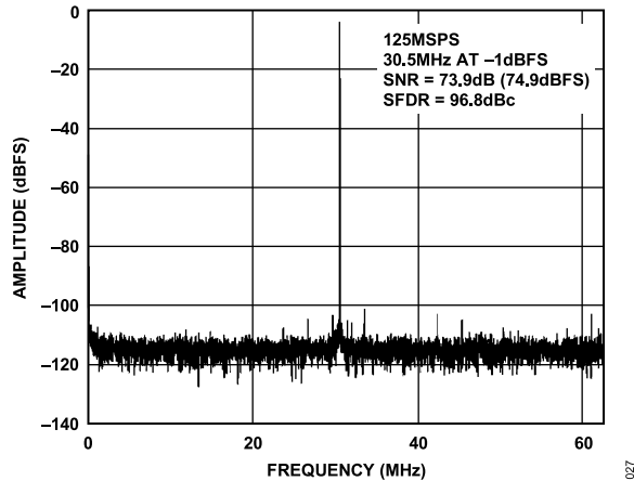
Figure 29. Single-Tone 16k FFT with f_{IN} = 30.5 MHz, f_{SAMPLE} = 125 MSPS
