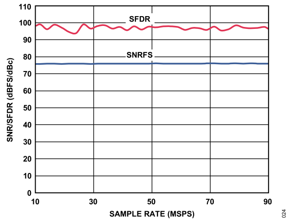
Figure 26. SNR/SFDR vs. Sample Rate; f_{IN} = 9.7 \text{ MHz} , f_{SAMPLE} = 80 \text{ MSPS}
