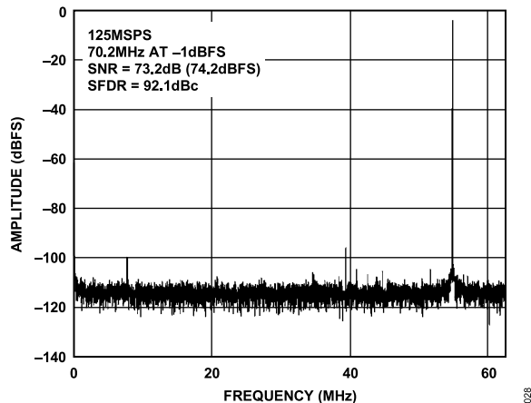
Figure 30. Single-Tone 16k FFT with f_{IN} = 70.2 MHz, f_{SAMPLE} = 125 MSPS
