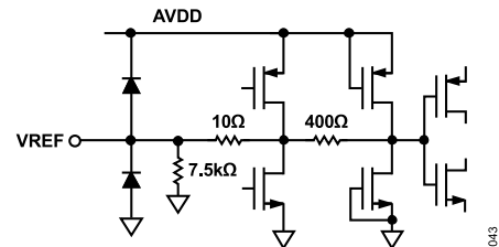
Figure 52. Equivalent VREF Circuit
