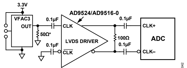
Figure 41. Differential LVDS Sample Clock
