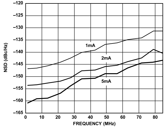
Figure 16. NSD vs. f_{OUT} and I_{OUTFS} at 175 MSPS
