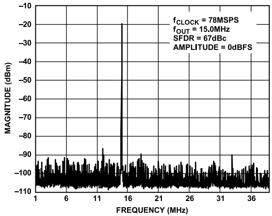
Figure 64. AD9704 Single-Tone SFDR
