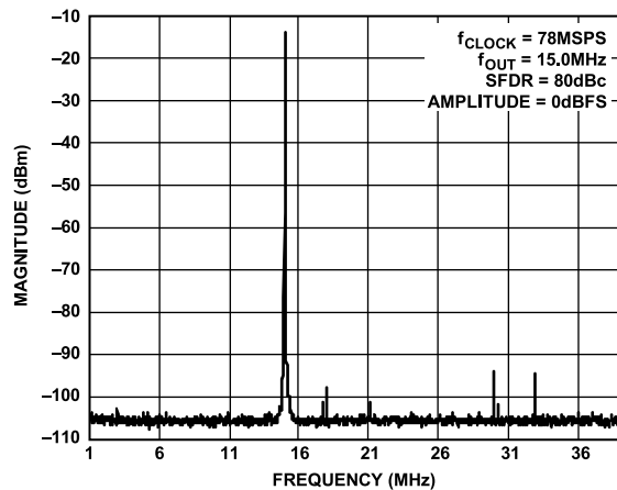
Figure 24. Single-Tone SFDR
