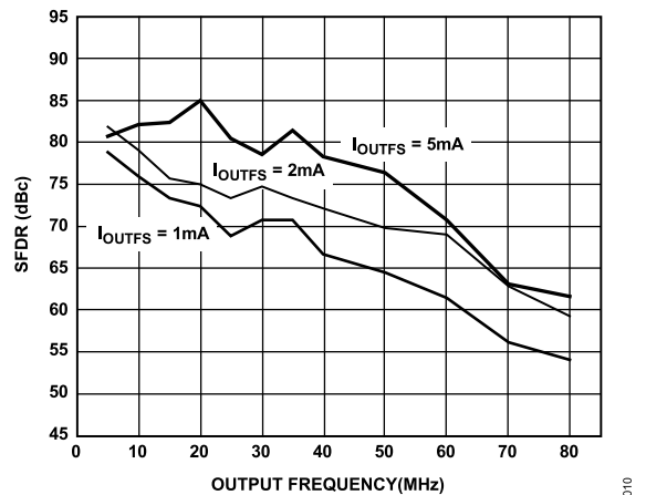
Figure 12. SFDR vs. f_{OUT} and I_{OUTFS} at 175 MSPS
