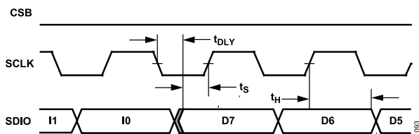
Figure 76. Timing Diagram for SPI Register Read
