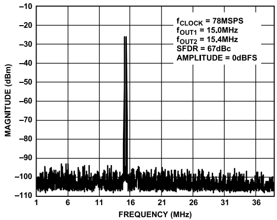
Figure 65. AD9704 Dual-Tone SFDR
