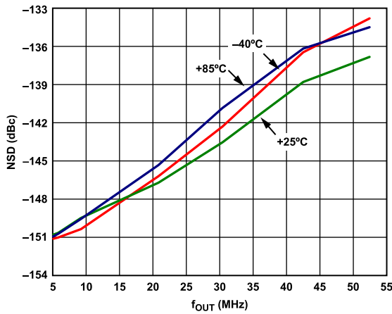
Figure 38. AD9717 Noise Spectral Density at Three Temperatures, 1.8 V
