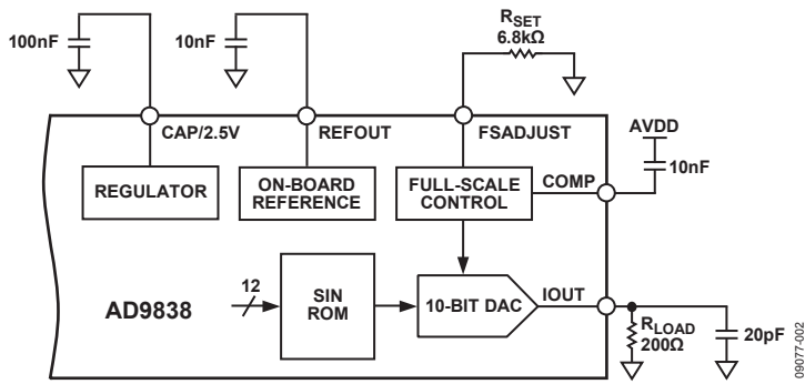
Figure 19. Test Circuit Used to Test Specifications
