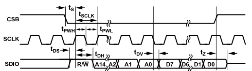
Figure 3. Timing Diagram for 3-Wire Read Operation
