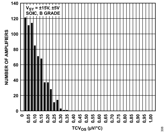
Figure 20. TCV_{OS} Distribution (SOIC, B Grade)
