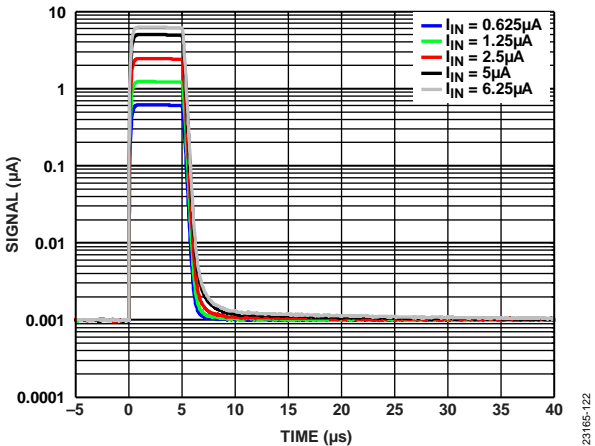
Figure 45. Settling Time for Various Input Currents, T_z = 200\text{ k}\Omega , 5 µs Pulse Width, LPF = 1 MHz
