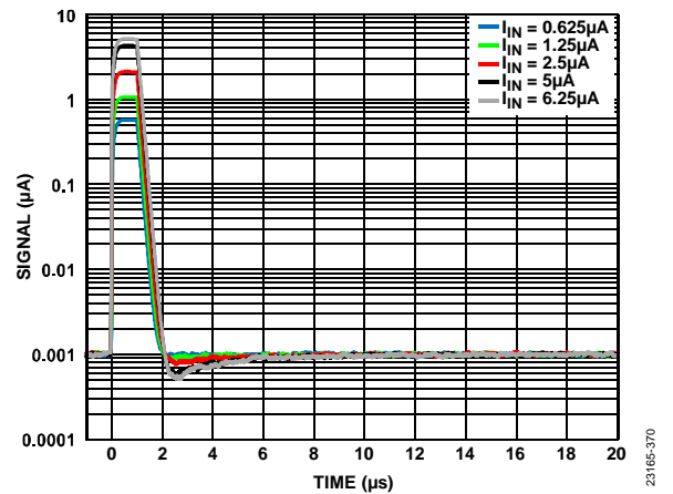
Figure 48. Settling Time for Various Input Currents, T_z = 200\text{ k}\Omega , 1 µs Pulse Width, LPF = 100 MHz
