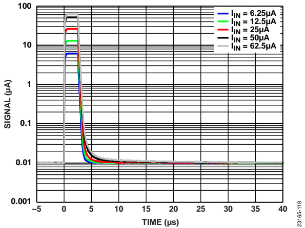
Figure 44. Settling Time for Various Input Currents, T_z = 20\text{ k}\Omega , 2.5 µs Pulse Width, LPF = 1 MHz
