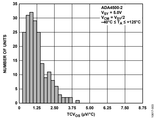
Figure 9. Input Offset Voltage Drift Distribution, V_{SY} = 5.0\text{ V}
