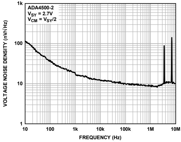
Figure 49. Voltage Noise Density vs. Frequency, V SY = 2.7 V (10 Hz to 10 MHz)
