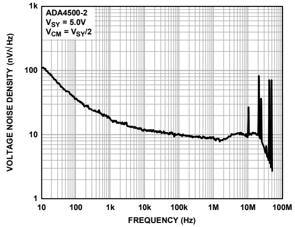
Figure 53. Voltage Noise Density vs. Frequency, V SY = 5.0 V (10 Hz to 100 MHz)
