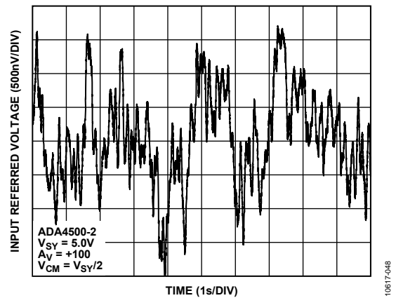
Figure 54. 0.1 to 10 Hz Noise, V SY = 5.0 V
