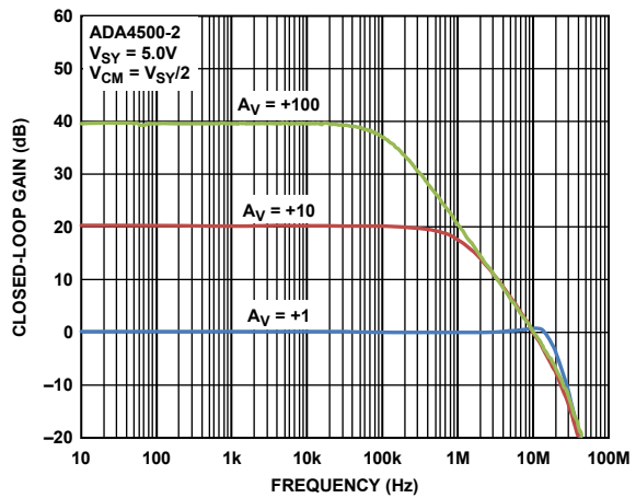
Figure 28. Closed-Loop Gain vs. Frequency, V SY = 5.0 V
