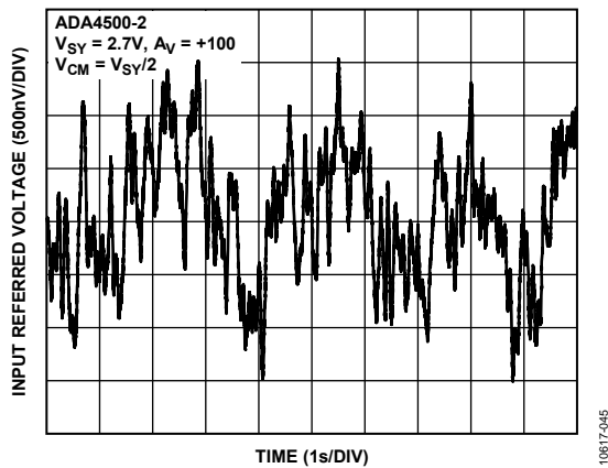
Figure 51. 0.1 to 10 Hz Noise, V SY = 2.7 V
