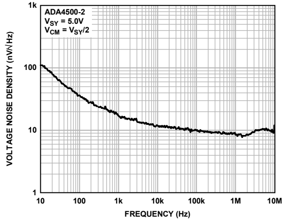
Figure 52. Voltage Noise Density vs. Frequency, V SY = 5.0 V (10 Hz to 10 MHz)
