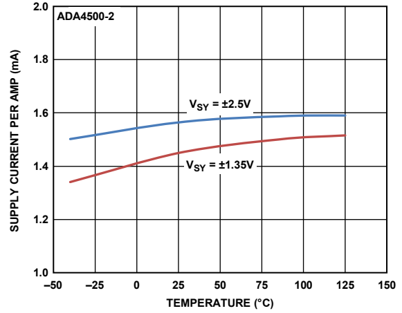
Figure 26. Supply Current per Amp vs. Temperature
