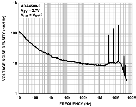
Figure 50. Voltage Noise Density vs. Frequency, V SY = 2.7 V (10 Hz to 100 MHz)
