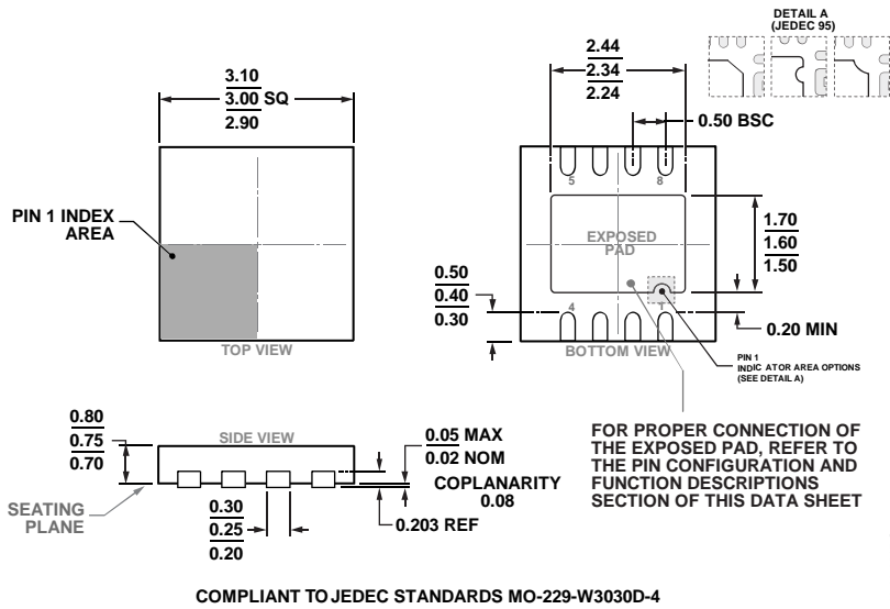
Figure 75. 8-Lead Lead Frame Chip Scale Package [LFCSP]
