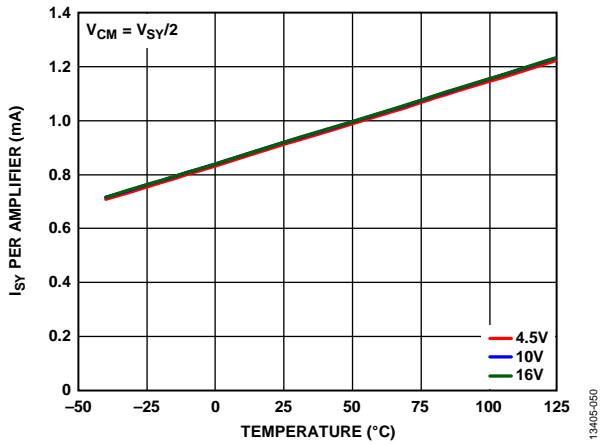
Figure 53. Supply Current ( I_{sv} ) per Amplifier vs. Temperature
