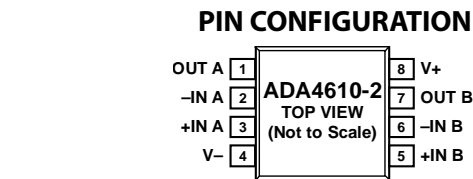
Figure 1. ADA4610-2 8-Lead SOIC (R Suffix); for Additional Packages and Models, See the Pin Configurations and Function Descriptions Section
