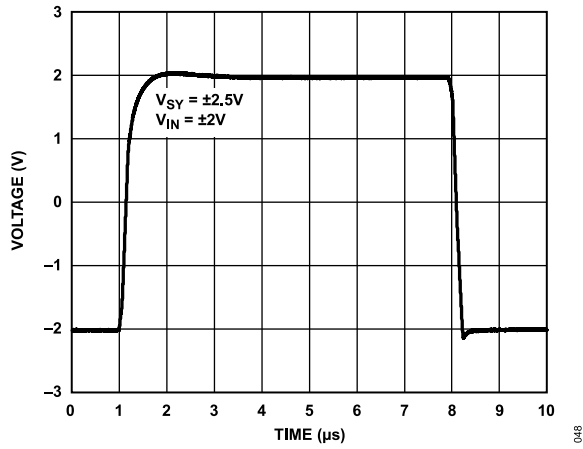
Figure 52. Large Signal Transient Response, V SY = ±2.5 V
