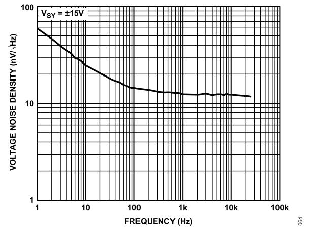
Figure 68. Voltage Noise Density, V_{SY} = \pm 15\text{ V}
