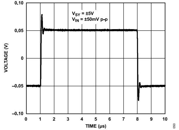
Figure 54. Small Signal Transient Response, V SY = ±5 V
