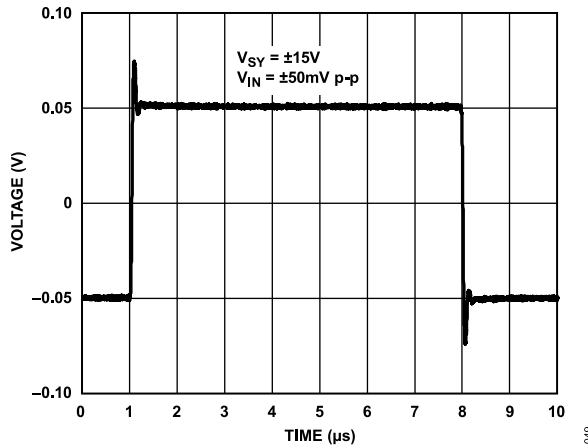
Figure 53. Small Signal Transient Response, V SY = ±15 V
