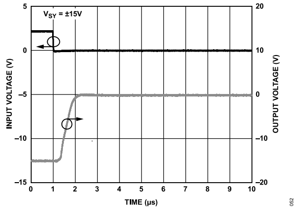
Figure 56. Negative Overload Recovery, A V = -10, V SY = ±15 V
