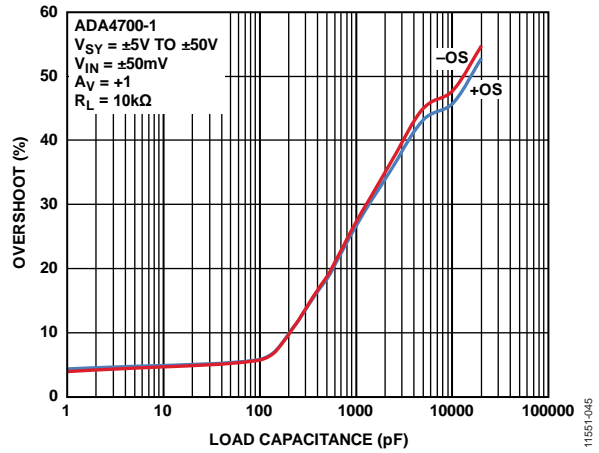
Figure 30. Small Signal Overshoot vs. Load Capacitance, V_{SY} = \pm 5 V to \pm 50 V
