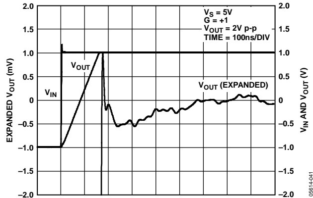
Figure 28. Settling Time
