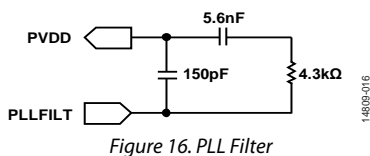
Figure 16. PLL Filter
