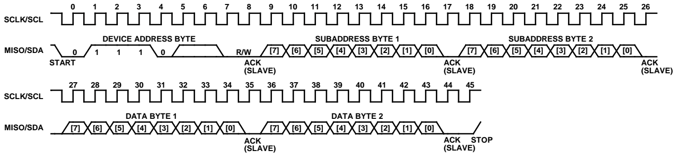
Figure 25. I 2 C Slave Single Word Write Operation (Two Bytes)
