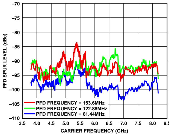
Figure 14. PFD Spurious Sweep, f_{PFD} = 61.44 \text{ MHz} , Loop Filter Bandwidth = 100 kHz
