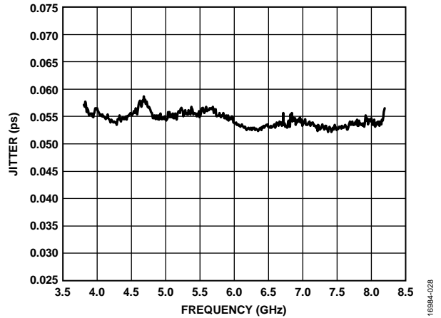
Figure 23. RMS Jitter Integrated from 1 kHz to 100 MHz, Fractional-N, f_{PFD} = 153.6 \text{ MHz} , V_{CC\_VCO} = 3.3 \text{ V}
