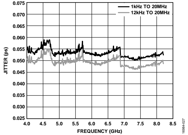
Figure 22. RMS Jitter, Fractional-N, f_{PFD} = 153.6 \text{ MHz} , V_{CC\_VCO} = 5 \text{ V}
