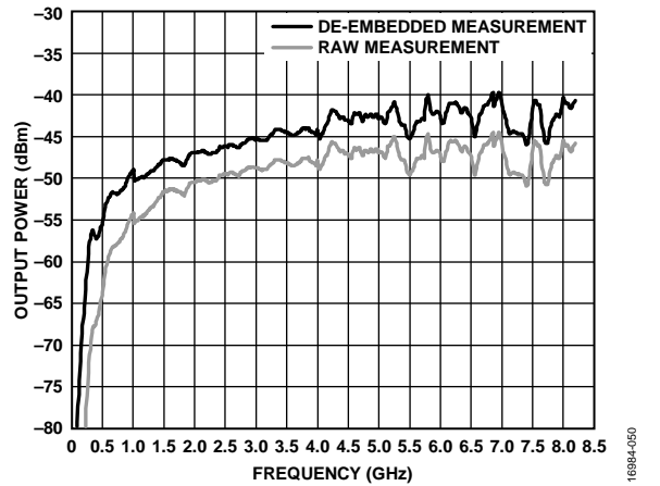
Figure 24. RF8P and RF8N Output Power When Disabled, De-Embedded Board and Cable Measurement, Combined Using Balun
