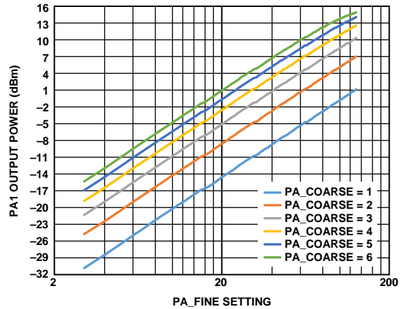
Figure 30. PA1 Output Power vs. PA_FINE Setting and PA_COARSE Setting with PA_FINE on a Logarithmic Scale, RF Frequency = 433 MHz, V_{DD} = 3.0 V , T_A = 25^\circ C
