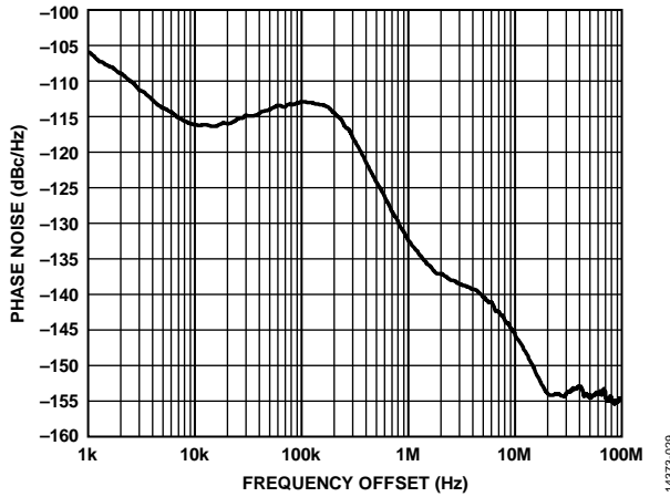
Figure 27. Phase Noise vs. Frequency Offset, RF Frequency = 433 MHz, PA1 Output Power = 10 dBm, V_{DD} = 3.0 V , T_A = 25^\circ C
