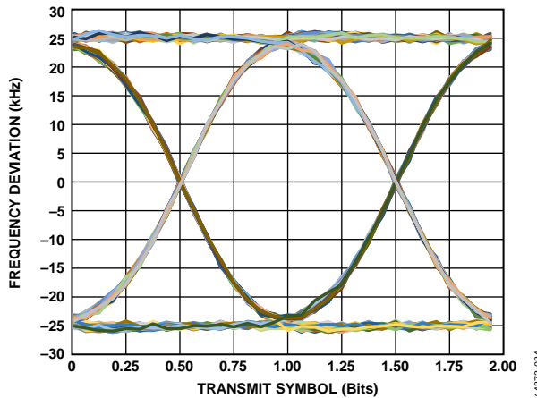
Figure 32. Transmit Eye Diagram, PA2 Output Power = 17 dBm, Configuration 433 MHz/50 kbps, V_{DD} = 3.0 V , T_A = 25^\circ C
