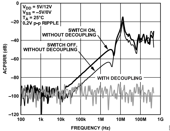
Figure 24. ACPSRR
