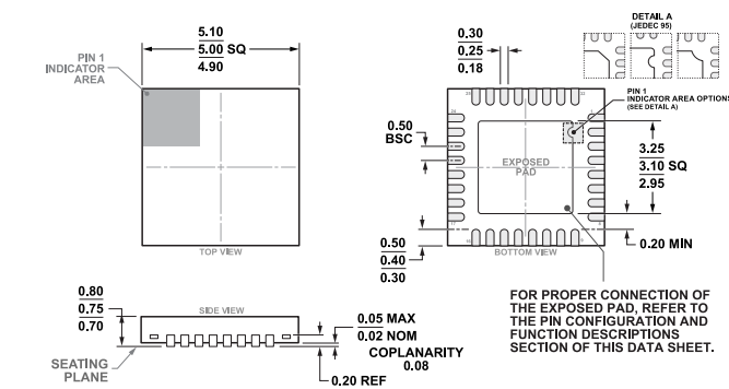
Figure 38. 32-Lead Lead Frame Chip Scale Package [LFCSP] 5 x 5 mm Body and 0.75 mm Package Height (CP-32-7) Dimensions shown in millimeters
