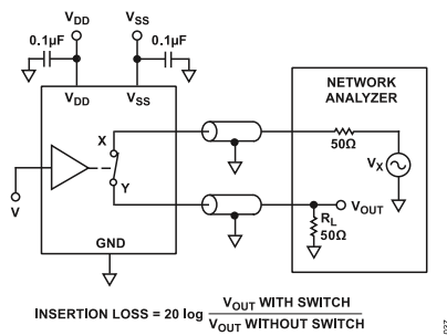
Figure 31. Bandwidth
