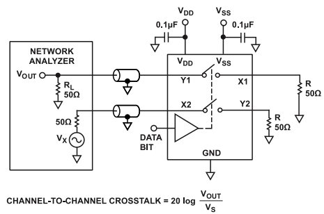
Figure 32. Channel-to-Channel Crosstalk
