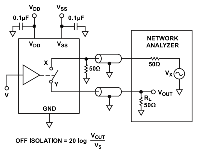
Figure 30. Off Isolation
