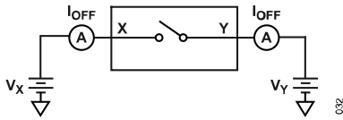
Figure 26. Off Leakage
