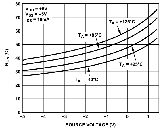
Figure 8. R_{ON} vs. Temperature, Dual \pm 5\text{ V} Supplies
