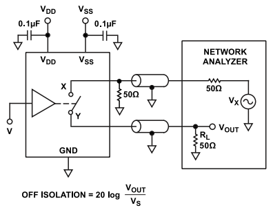
Figure 30. Off Isolation
