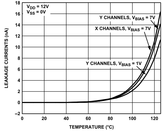
Figure 13. On Leakage vs. Temperature, 12 V Single Supply
