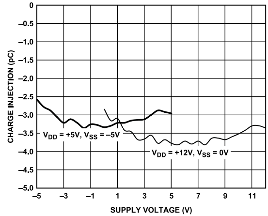
Figure 15. Charge Injection vs. Supply Voltage
