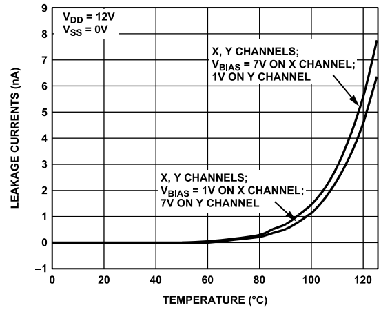
Figure 14. Off Leakage vs. Temperature, 12 V Single Supply
