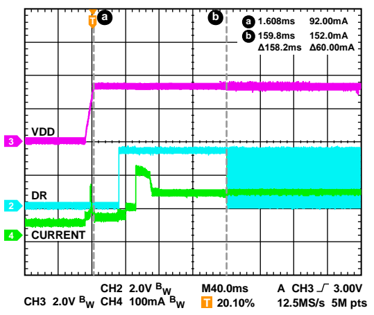
Figure 48. Transient Current Demand, Startup (DR Means Data Ready)
