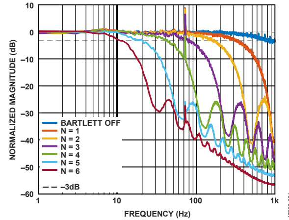
Figure 28. Accelerometer Normalized Noise Density
