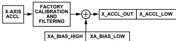
Figure 57. User Calibration Signal Path, Accelerometers
