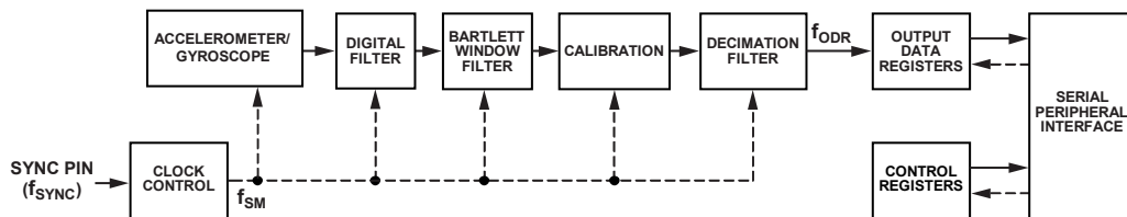
Figure 30. Sensor Signal Chain
