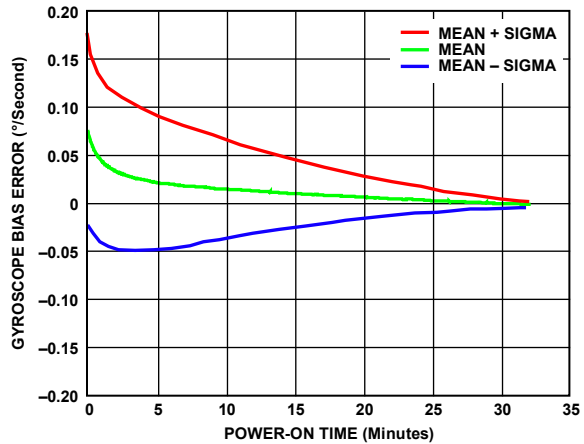
Figure 18. Gyroscopic Bias Error vs. Power-On Time, T_c = 85^\circ\text{C} , All Axes
