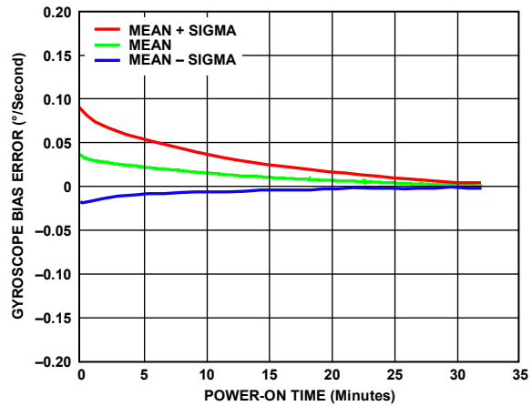
Figure 17. Gyroscopic Bias Error vs. Power-On Time, T_c = 25^\circ\text{C} , All Axes
