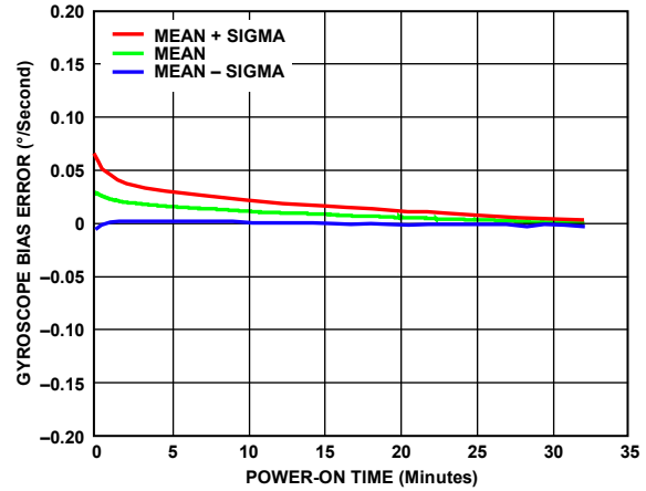
Figure 16. Gyroscopic Bias Error vs. Power-On Time, T_c = -40^\circ\text{C} , All Axes
