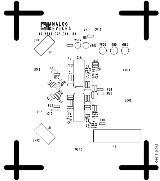
Figure 42. Component-Side Silkscreen
