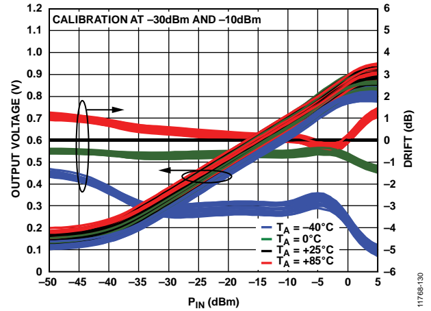
Figure 30. Distribution of Log Conformance Error with Respect to V_{LOG} at 25°C vs. P_{IN} and Temperature at 4500 MHz
