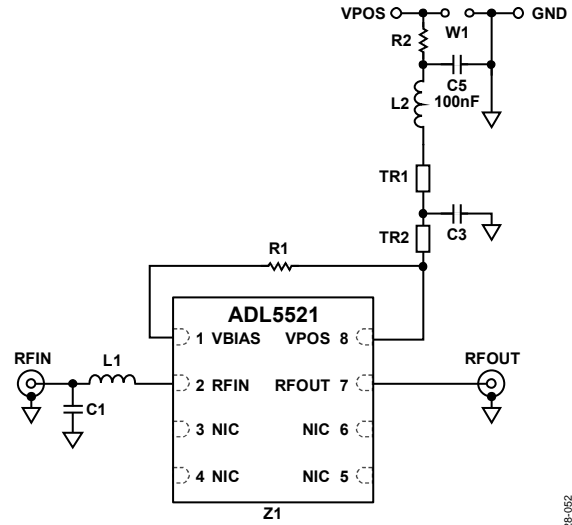
06828-052 NIC = NO INTERNAL CONNECTION. DO NOT CONNECT TO THIS PIN.
