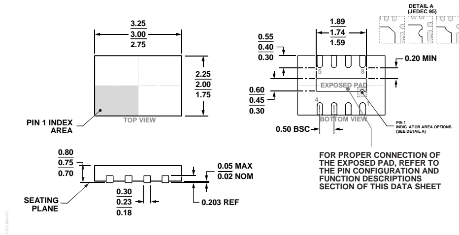
Figure 28. 8-Lead Lead Frame Chip Scale Package [LFCSP] 2 mm × 3 mm Body and 0.75 mm Package Height (CP-8-23) Dimensions shown in millimeters
