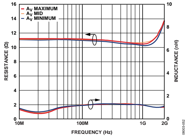
Figure 31. Output Resistance and Inductance vs. Frequency
