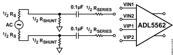
Figure 38. Gain Adjustment Using a Series Resistor
