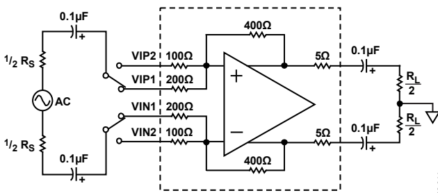
Figure 35. Differential Input Loading Circuit
