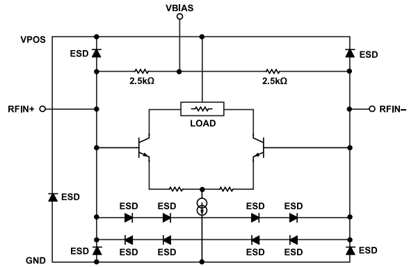
Figure 42. RF Inputs
