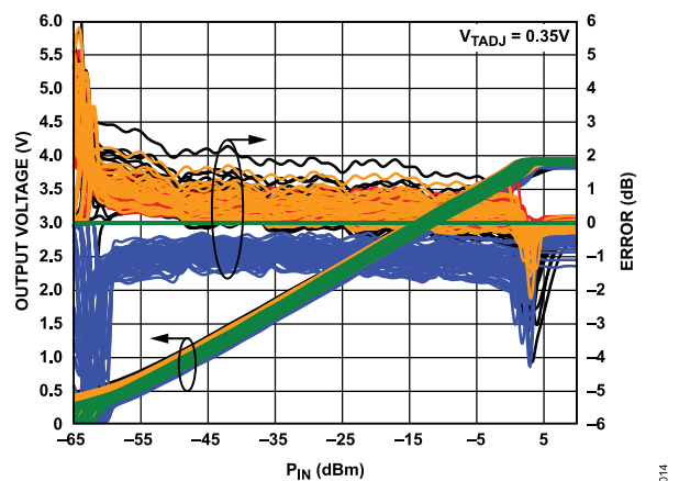
Figure 14. Distribution of Log Conformance Error with Respect to V_{RMS} at 25°C vs. Input Level and Temperature at 900 MHz
