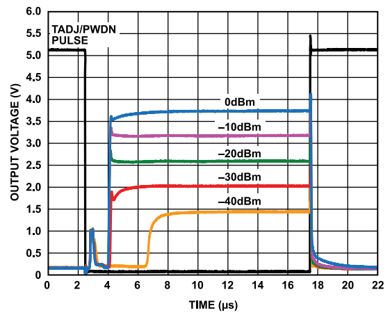
Figure 31. Output Response Using Power-Down Mode for Various RF Input Levels, Carrier Frequency = 2.14 GHz, C_{RMS} = 1 nF
