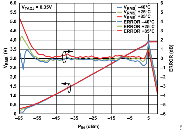
Figure 58. V_{RMS}' and Log Conformance Error vs. Input Level and Temperature at 1900 MHz Using V_{TEMP} Intercept Compensation
