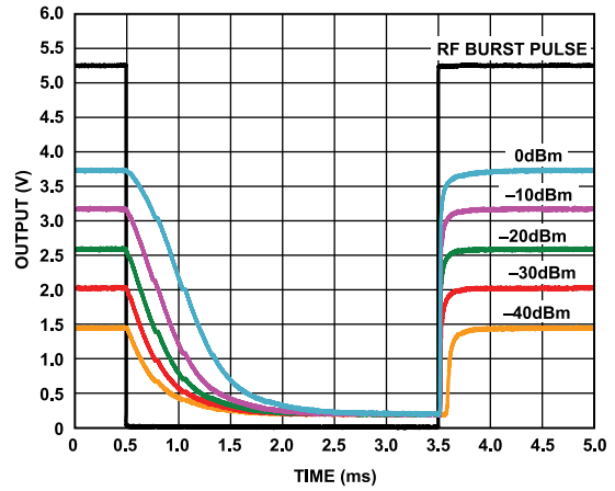
Figure 30. Output Response to RF Burst Input, Carrier Frequency = 2.14 GHz
