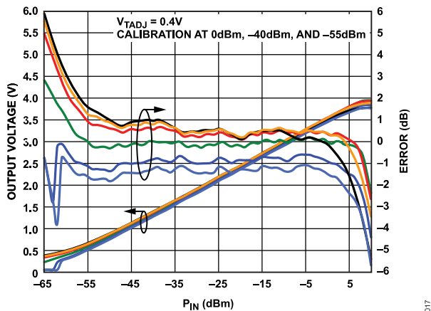
Figure 17. V_{RMS} and Log Conformance Error vs. Input Level and Temperature at 2.6 GHz
