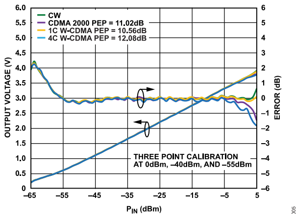
Figure 5. Error from CW Linear Reference vs. Signal Modulation (CDMA 2000, One-Carrier W-CDMA, Four-Carrier W-CDMA), Frequency = 2.14 GHz
