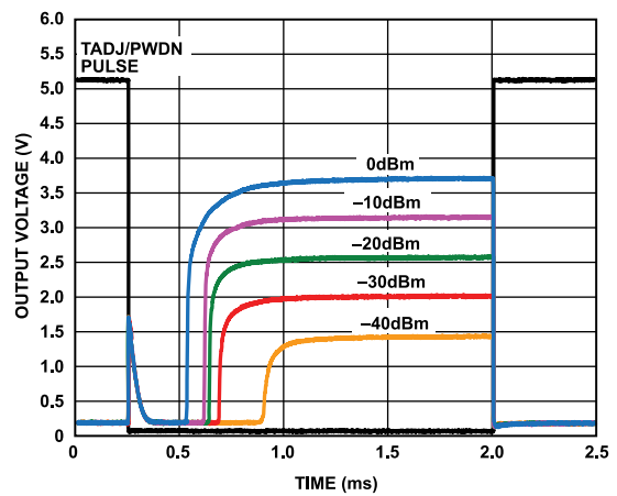
Figure 32. Output Response Using Power-Down Mode for Various RF Input Levels, Carrier Frequency = 2.14 GHz
