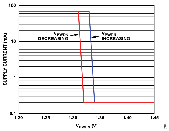
Figure 38. Supply Current vs. V_{PWDN}
