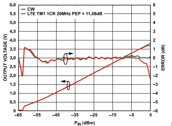
Figure 8. Error from CW Linear Reference vs. Signal Modulation (LTE TM1 One-Carrier, 20 MHz), Frequency = 2.14 GHz, Three Point Calibration at 0 dBm, -40 dBm, and -55 dBm
