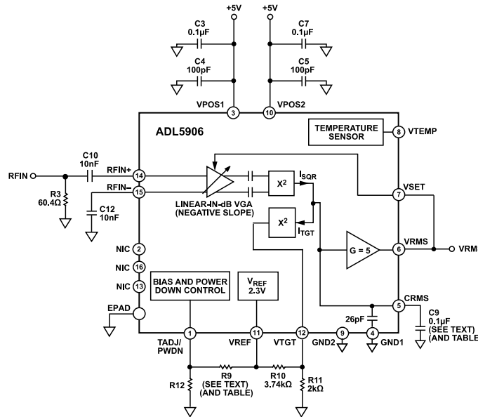
Figure 51. Basic Connections for Operation in Measurement Mode
