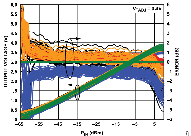
Figure 20. Distribution of Log Conformance Error with Respect to V_{RMS} at 25°C vs. Input Level and Temperature at 2.6 GHz
