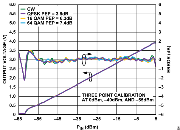
Figure 4. Error from CW Linear Reference vs. Signal Modulation (QPSK, 16 QAM, 64 QAM), Frequency = 900 MHz
