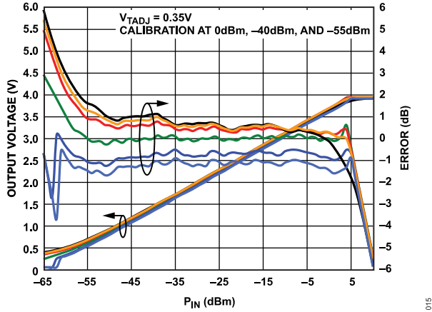
Figure 15. V_{RMS} and Log Conformance Error vs. Input Level and Temperature at 1.9 GHz
