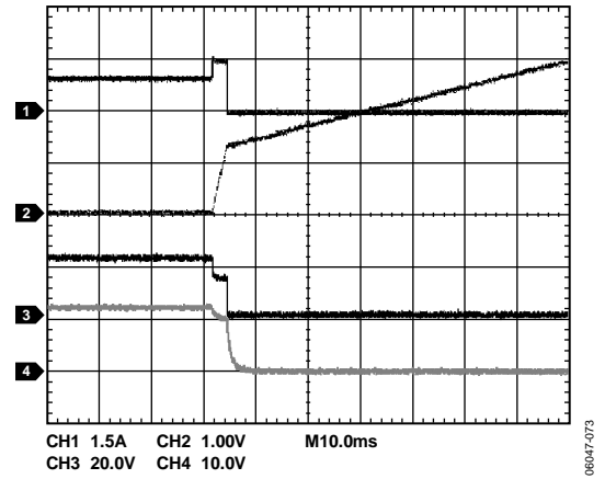
Figure 46. Overcurrent Condition During Operation (ADM1177-1 Model) (Channel 1 = I_{LOAD} , Channel 2 = V_{TIMER} , Channel 3 = V_{GATE} , Channel 4 = V_{OUT} )
