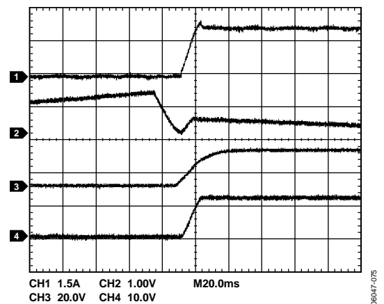
Figure 48. Inrush Current Control with Profiling of Initial Current Edge via a Capacitor on the SS Pin (Channel 1 = I_{LOAD} , Channel 2 = V_{TIMER} , Channel 3 = V_{GATE} , Channel 4 = V_{OUT} )
