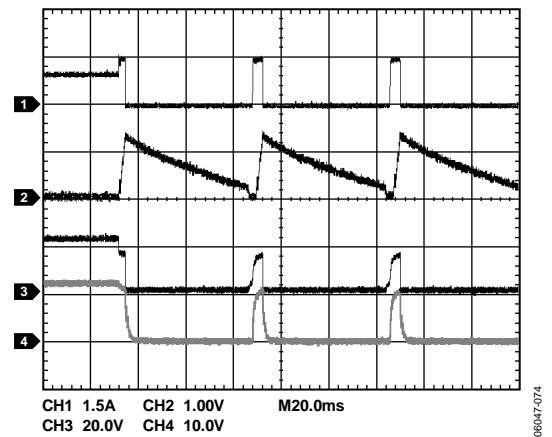
Figure 47. Overcurrent Condition During Operation (ADM1177-2 Model) (Channel 1 = I_{LOAD} , Channel 2 = V_{TIMER} , Channel 3 = V_{GATE} , Channel 4 = V_{OUT} )
