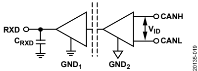
Figure 18. Receiver Voltage Measurement
