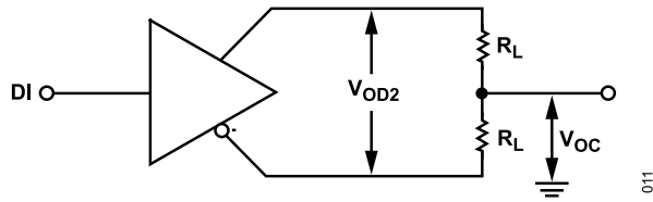
Figure 38. Driver Voltage Measurements
