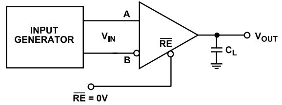
Figure 42. Receiver Propagation Delay/Skew
