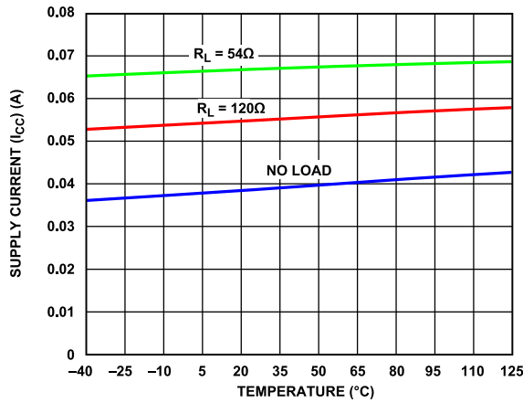
Figure 16. Supply Current ( I_{CC} ) vs. Temperature, Data Rate = 50 Mbps, 50 Mbps Models, V_{CC} = 3.3\text{ V}
