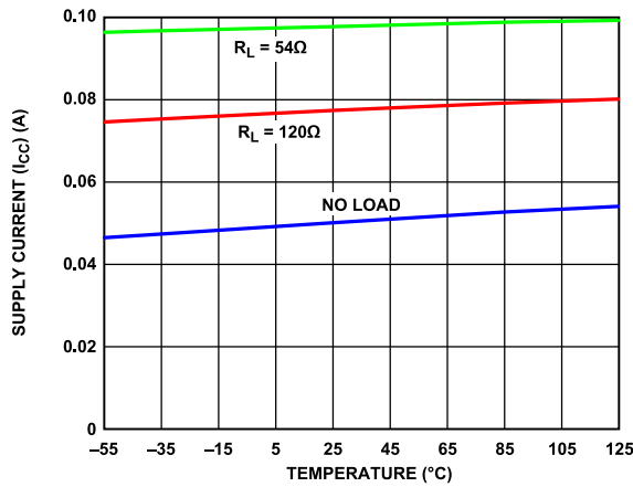
Figure 17. Supply Current ( I_{CC} ) vs. Temperature, Data Rate = 50 Mbps, 50 Mbps Models, V_{CC} = 5.0\text{ V}
