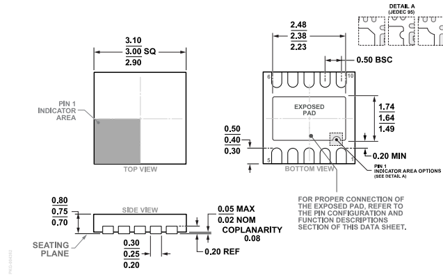
Figure 53. 10-Lead Lead Frame Chip Scale Package [LFCSP] 3 mm x 3 mm Body and 0.75 mm Package Height (CP-10-9)
