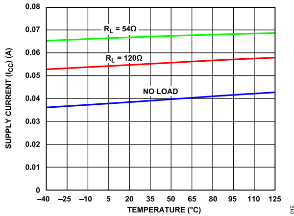
Figure 16. Supply Current ( I_{CC} ) vs. Temperature, Data Rate = 50 Mbps, 50 Mbps Models, V_{CC} = 3.3\text{ V}
