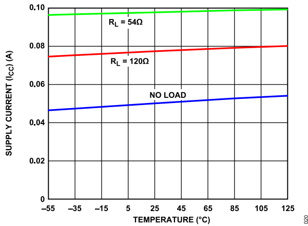
Figure 17. Supply Current ( I_{CC} ) vs. Temperature, Data Rate = 50 Mbps, 50 Mbps Models, V_{CC} = 5.0\text{ V}
