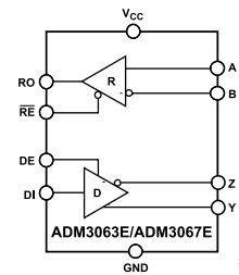
Figure 2. ADM3063E/ADM3067E Functional Block Diagram
